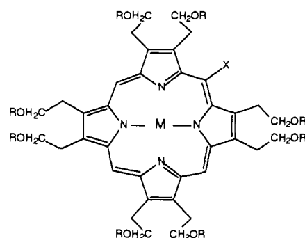
Figure 1. Schematic synthesis of octaethanolporphyrin ( H_2(EtOH)_8Por ) and its octaether derivatives ( H_2(ETOR)_8Por ): (a) HCl; (b) 2,4-pentanedione/ Zn/AcOH/ca. 75\text{ }^\circ\text{C} ; (c) Ti(NO_3)_3/MeOH/HClO_4 ; (d) NaOMe/MeOH; (e) BH_3/THF ; (f) TsCl/pyridine; (g) ROH/toluene; (h) Pb(OAc)_2 ; (i) KOH/EtOH; (j) HBr/EtOH; (k) chloranil; (l) AcCl/ NEt_3 ; (m) O_2 .
