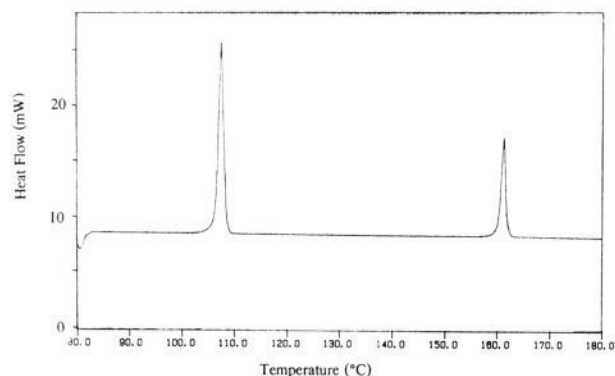
Figure 3. Differential scanning calorimogram of Zn(EtOOct) 8 Por ( 14b ). Endothermic transitions are plotted upward.
