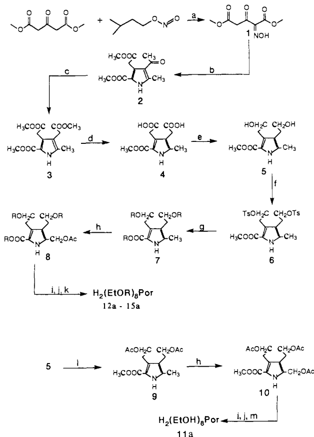
Figure 1. Schematic synthesis of octaethanolporphyrin ( H_2(EtOH)_8Por ) and its octaether derivatives ( H_2(ETOR)_8Por ): (a) HCl; (b) 2,4-pentanedione/ Zn/AcOH/ca. 75\text{ }^\circ\text{C} ; (c) Ti(NO_3)_3/MeOH/HClO_4 ; (d) NaOMe/MeOH; (e) BH_3/THF ; (f) TsCl/pyridine; (g) ROH/toluene; (h) Pb(OAc)_2 ; (i) KOH/EtOH; (j) HBr/EtOH; (k) chloranil; (l) AcCl/ NEt_3 ; (m) O_2 .
